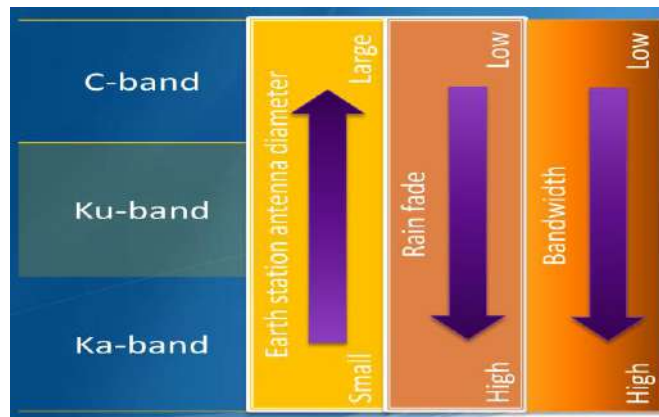
Figure 3.3: Technical Characteristics of higher spectrum bands 17
