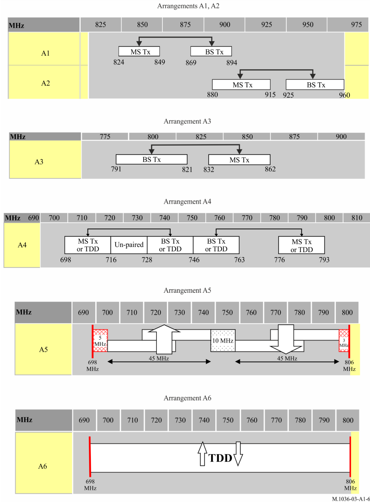
FIGURE 3 Frequency arrangements A1 to A13 (see NOTES to Table 2)
